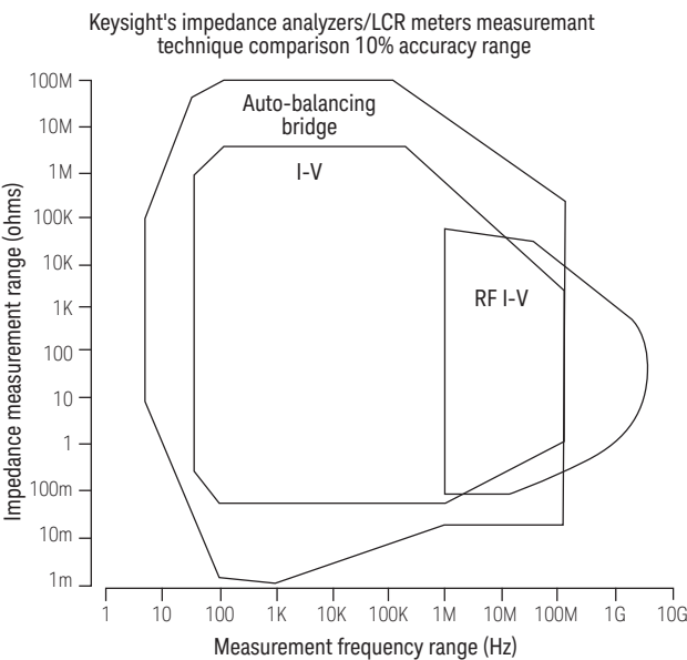
Figure 1. Impedance measurement techniques of impedance analyzers/ LCR meters
