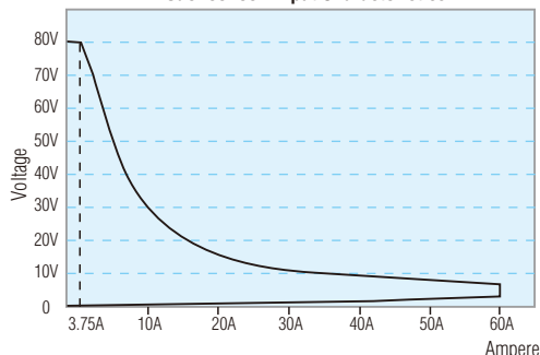
Low Voltage Characteristics (Typical)
