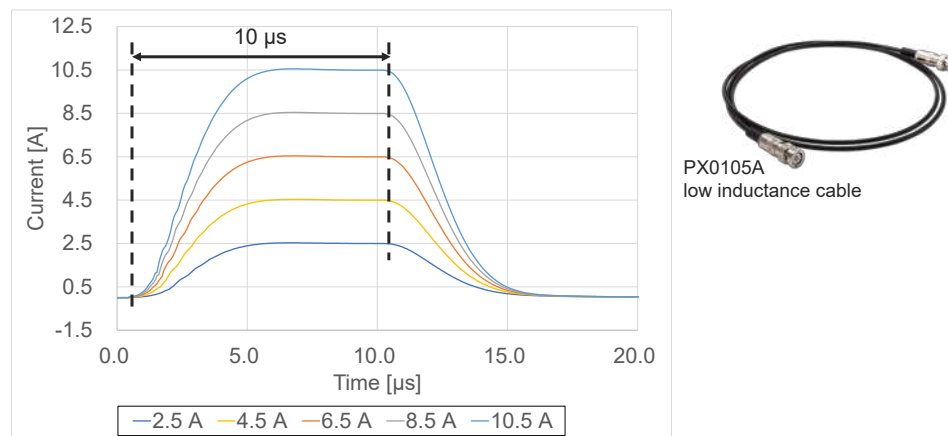
Figure 9. 10 \mu s narrow pulse output with measuring at 15 MSa/s sampling rate
