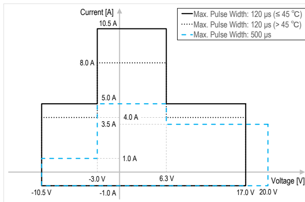
Figure 18. PZ2120/21A pulsed voltage and current output capability
