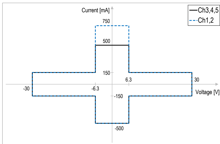
Figure 19. PZ2130/31A voltage and current output capability per channel
